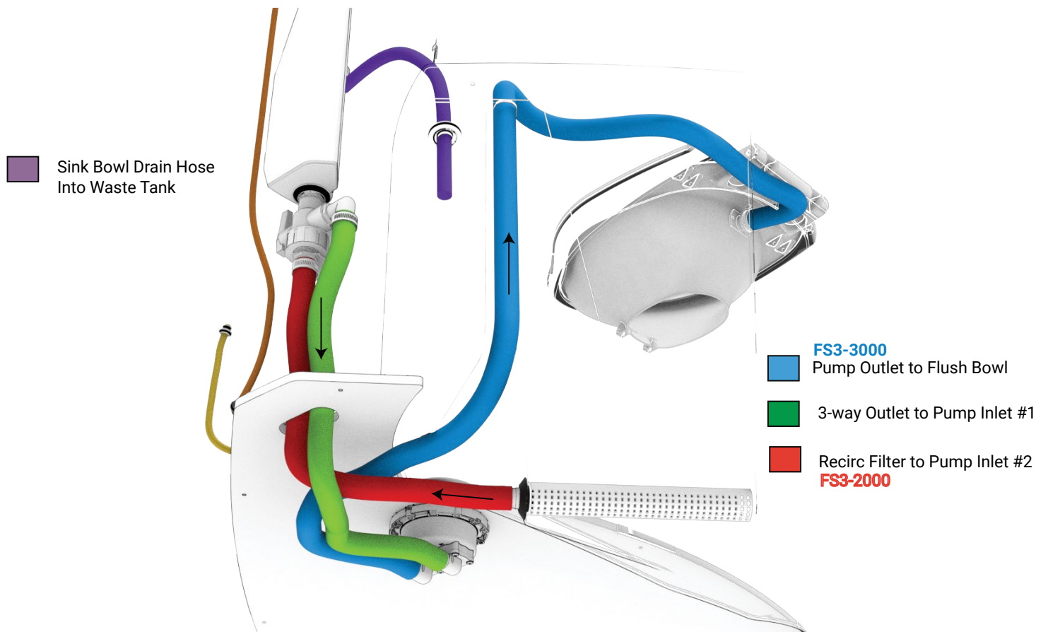
FS3-2000/3000 Flush Hose Connections with 3-Way Valve Installed.
