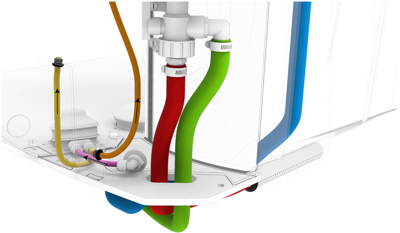
FS3-2000/3000 Flush Hose Connections with 3-Way Valve Installed.
